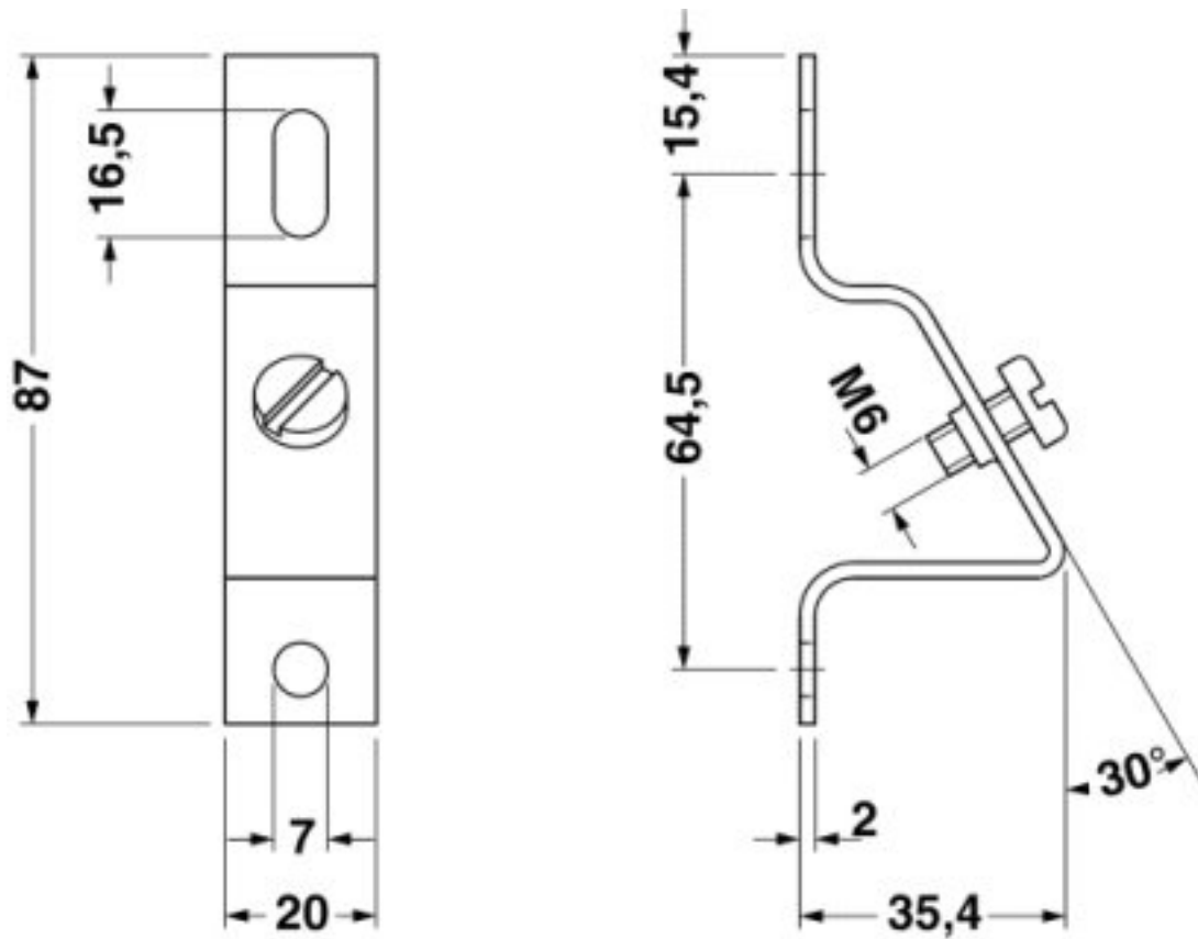
Dimensioned drawing
