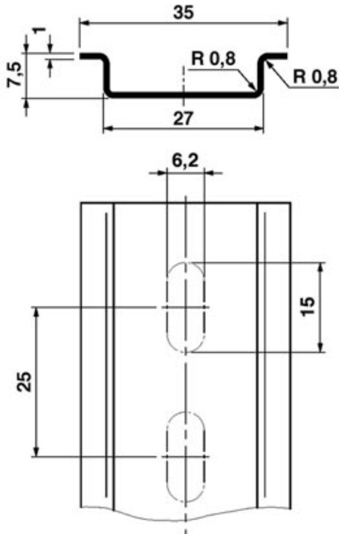
Dimensioned drawing
