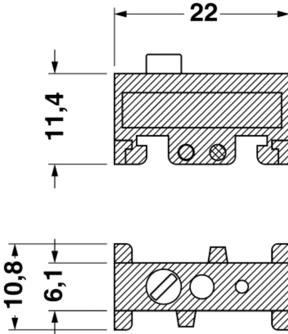
Dimensioned drawing
