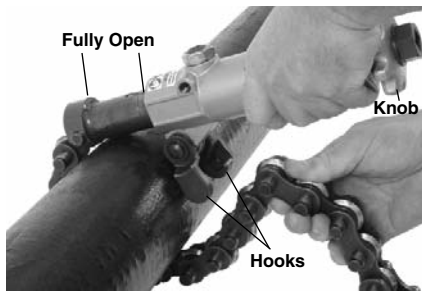
Figure 3 – Cutter Fully Open, Hooking the Chain
