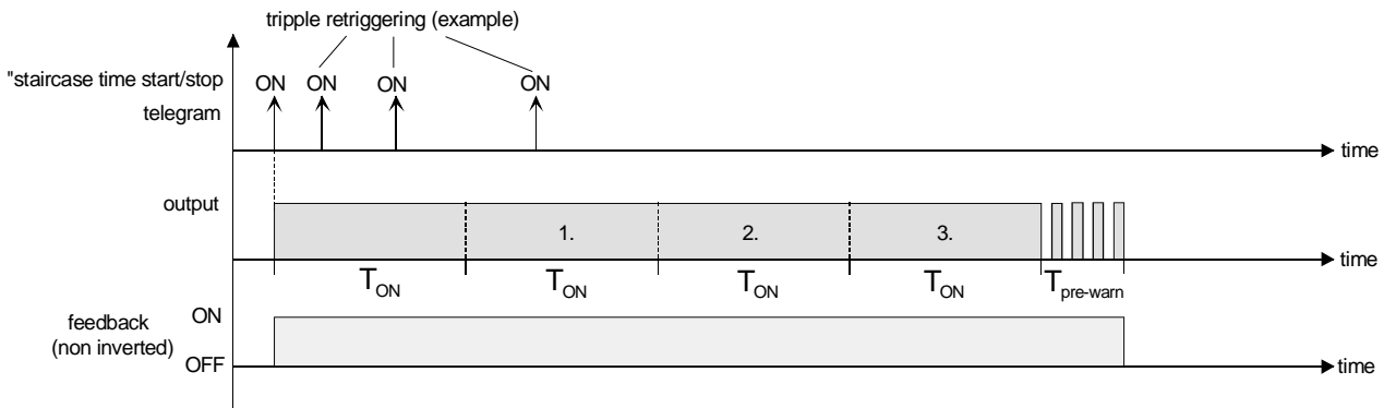
Fig. 14: Time extension for staircase lighting function
