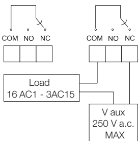
M2M ALARM electromechanical relay outputs
