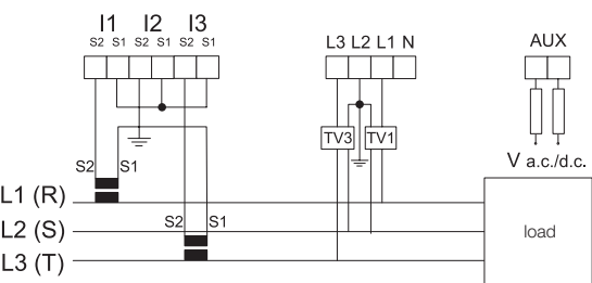
ARON Three-phase with 2 CT and 2 VT
