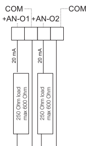
M2M I/O analogue outputs
