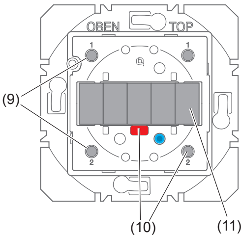
Figure 4: Wall-transmitter solar
