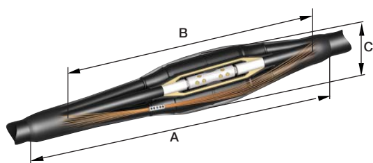
SOJ with cold-shrink outer jacket.
