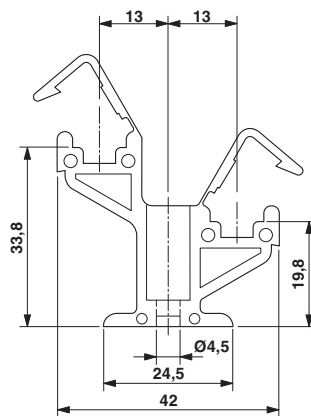
Dimensioned drawing
